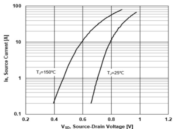
Figure 7. Source-Drain Diode Forward Characteristics
